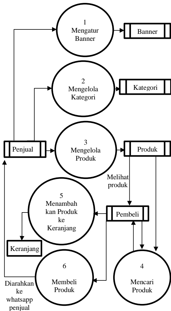
Gambar 5 Data Flow Diagram Level 1
