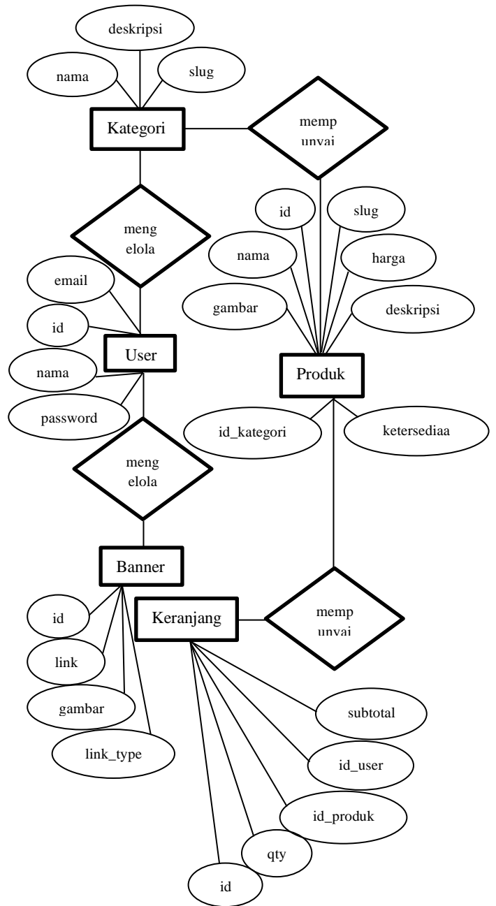
Gambar 6 Entity Relationship Diagram
